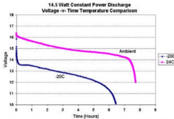
The internal resistance of a battery pack suppresses the voltage during discharge at low temperature (-20C) when compared to ambient (24C), resulting in reduced runtime.
